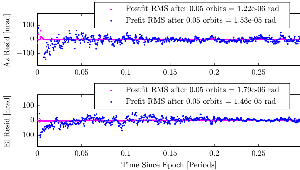
Figure 6.8: Estimation pre- and post-fit residuals for the curvilinear LROE set.
